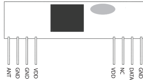
Figure 1 CY33 Shape & Pins
