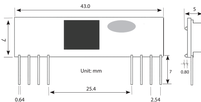
Figure 2 CY33 Dimension
