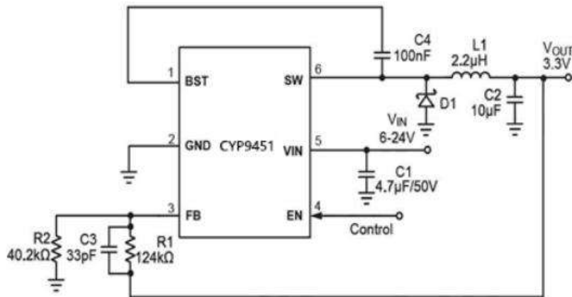
3.3V output typical application circuit
