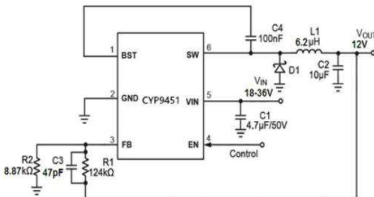
12V output typical application circuit
