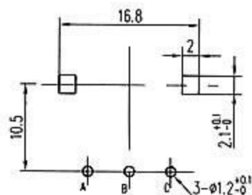
P.C.B MOUNTING DETAIL
