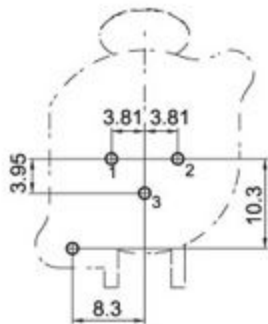
P.C.B LAYOUT (VIEWED FROM COPPER SIDE)
