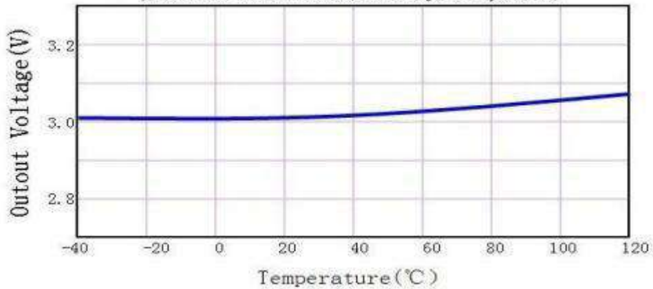
CY7330-APR Cin=CL=10uF (Electrolytic Capacitor)
