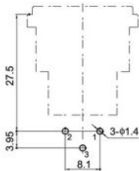
P.C.B LAYOUT (VIEWED FROM COPPER SIDE)
