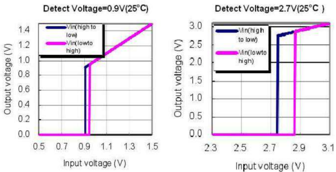
(1) Output Voltage vs Input voltage
